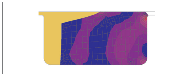
Merkel Cover Seal PU 83 at an operating pressure of 40 MPa
