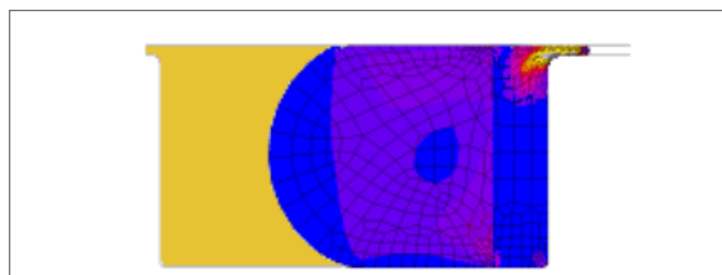
O-ring with a PTFE back-up ring at an operating pressure of 40 MPa
